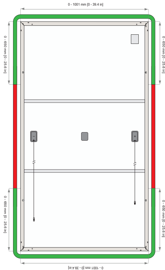
Fig. 29: REC 72-cell panels MLPE device installation zones
